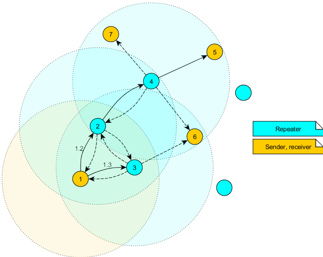
Figure 7: Example network
